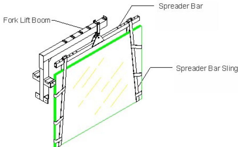
Spreader Bar shown with optional Slings & Fork Lift Boom
